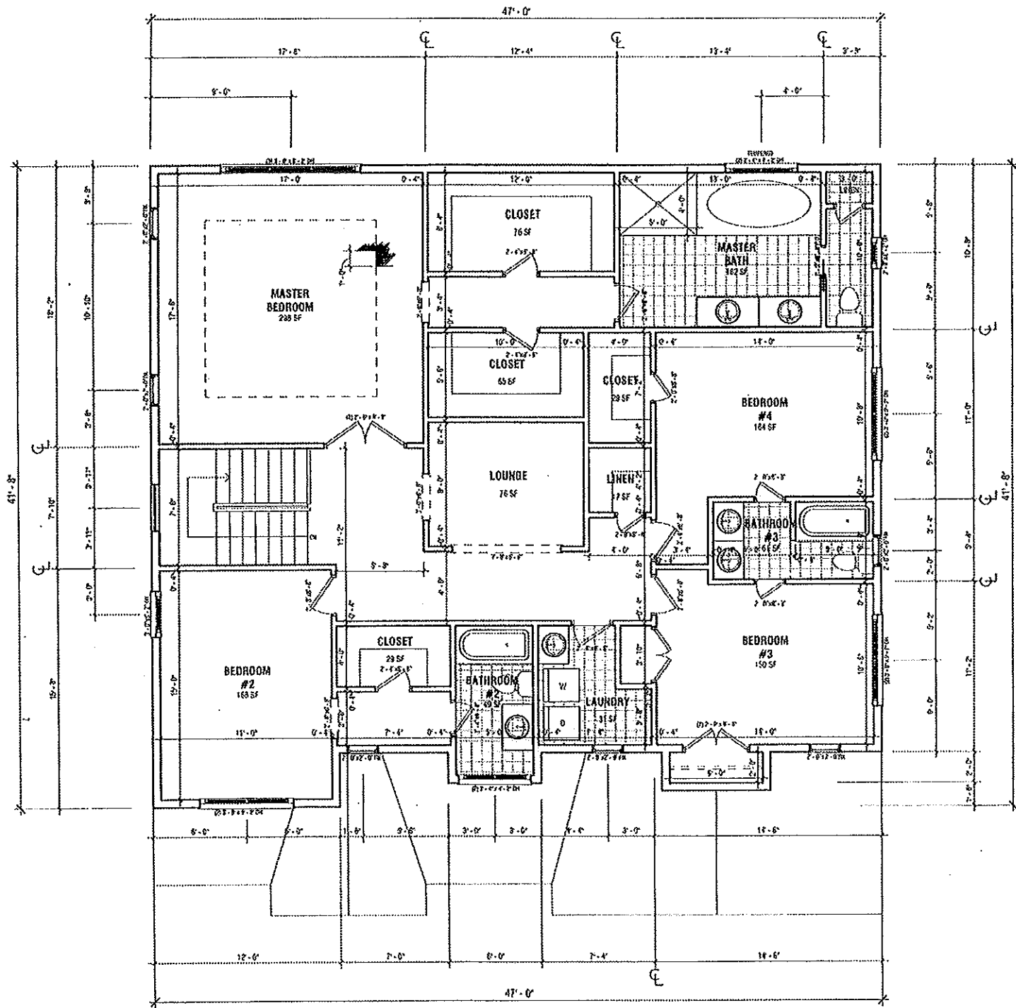
UPPER FLOOR 1844 SF
