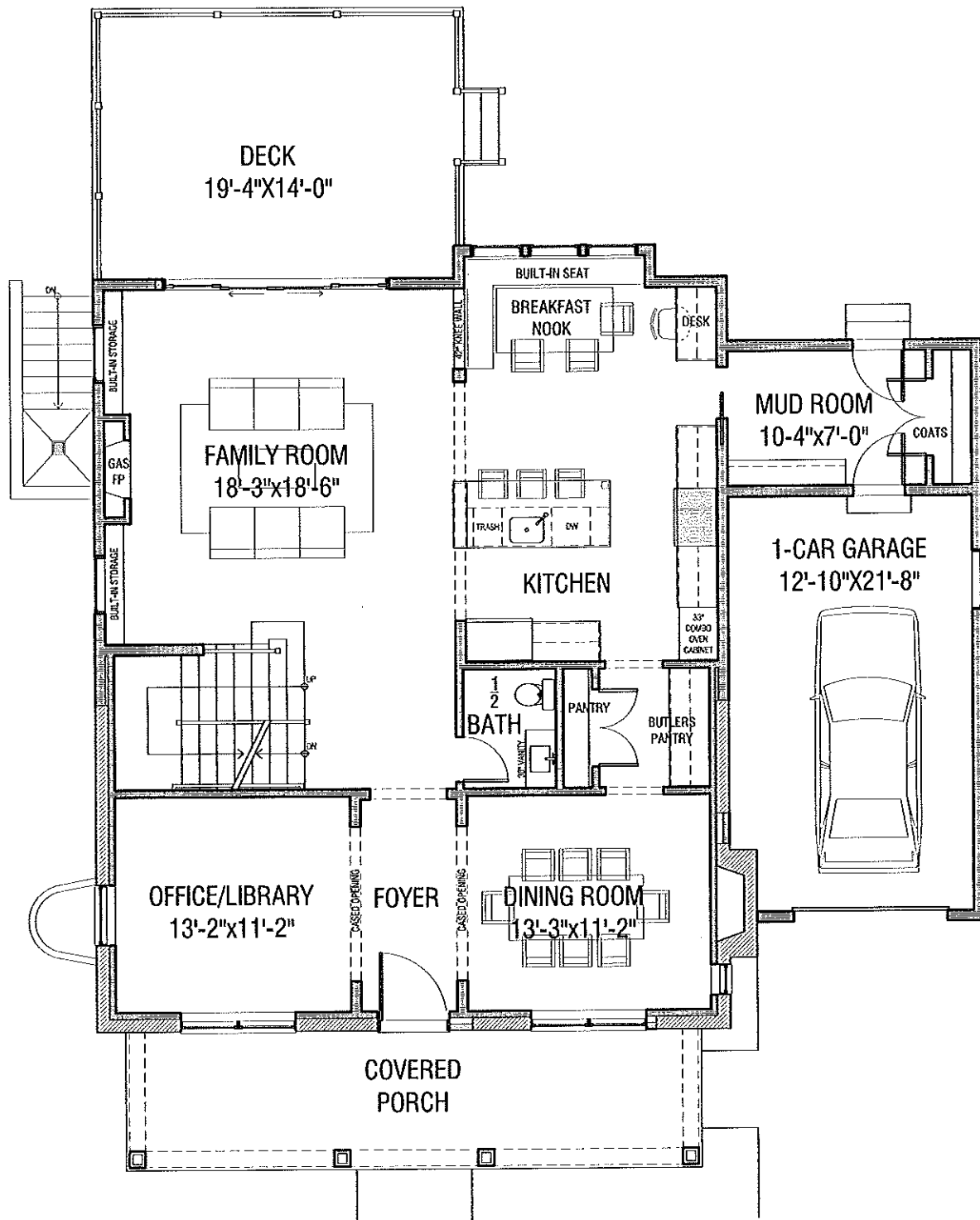
GROUND FLOOR PLAN - 1,412 S.F.
