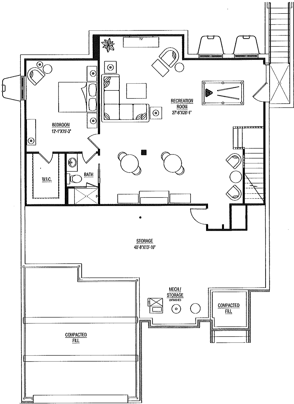
BASEMENT PLAN
