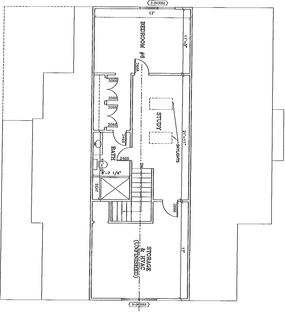
ATTIC FLOOR PLAN 1/4"=1'-0"
