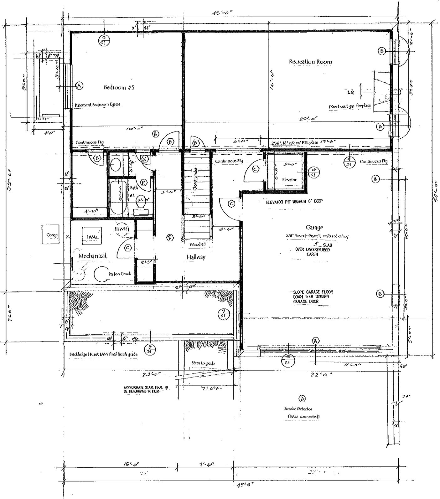
Basement Plan
