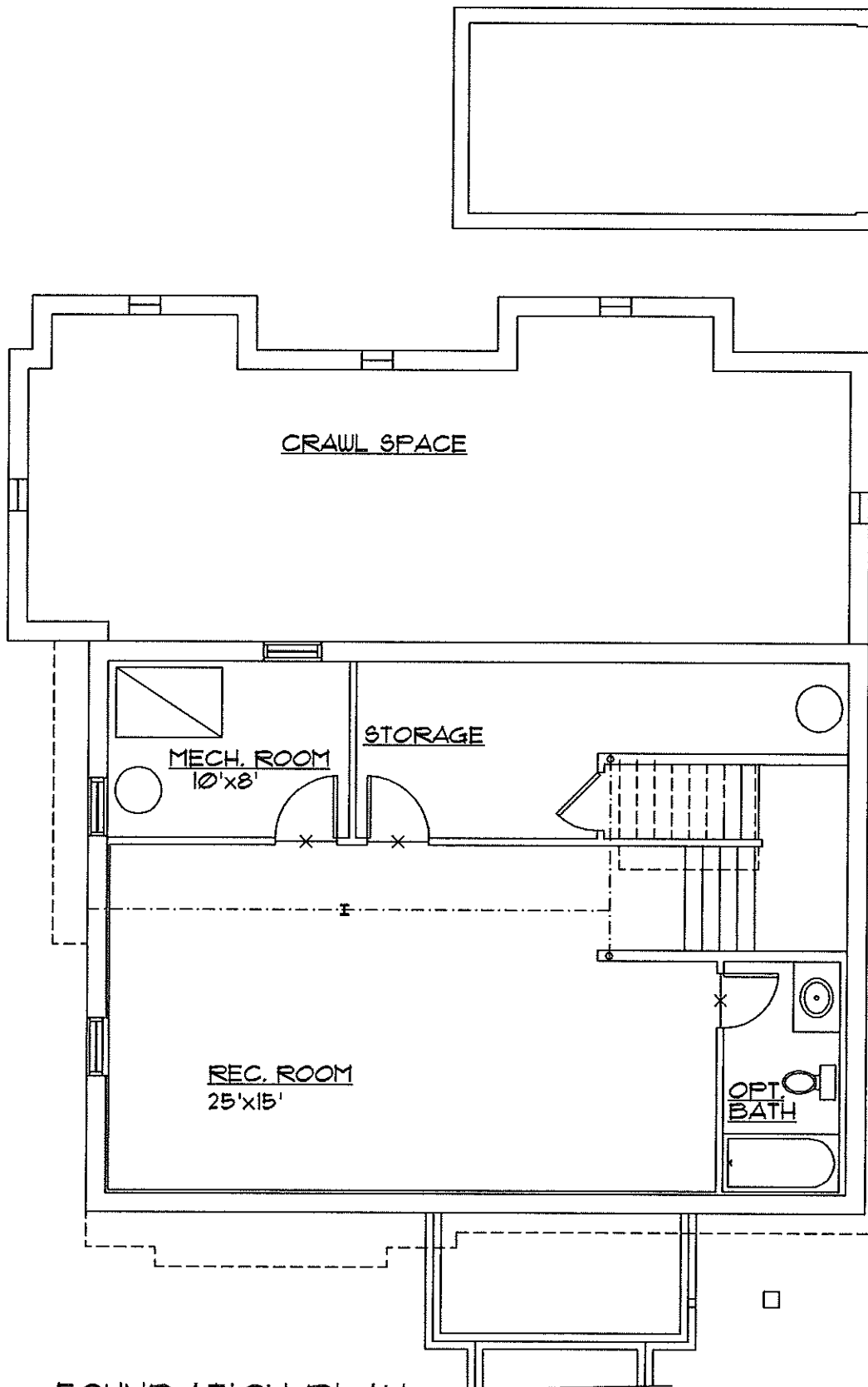
FOUNDATION PLAN
