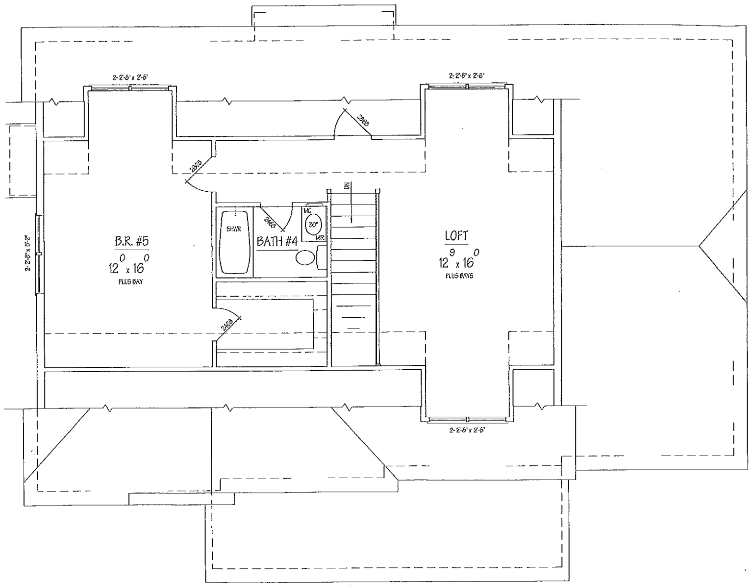
THIRD FLOOR PLAN 1/4"=1'-0"
