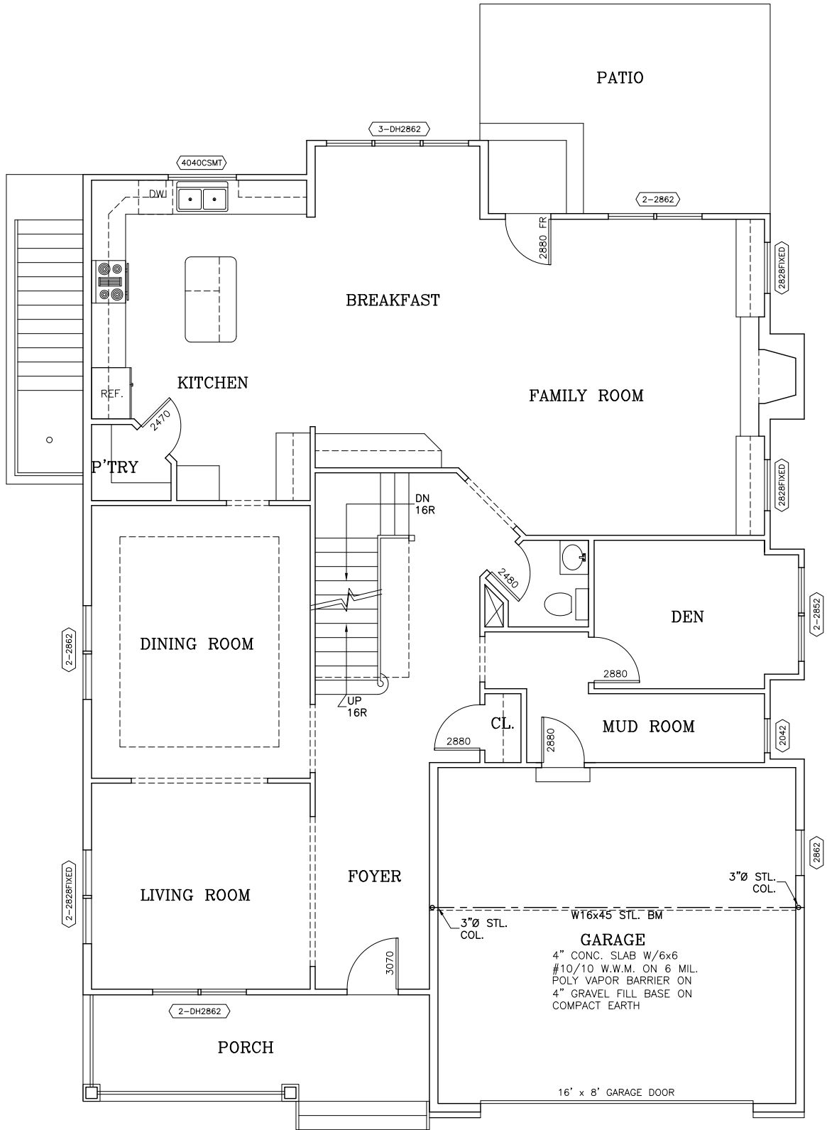
FIRST FLOOR PLAN 1/4"=1'-0"
