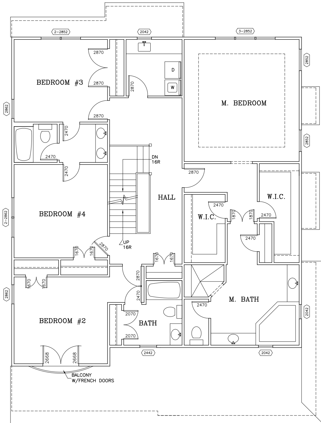
SECOND FLOOR PLAN 1/4"=1'-0"
