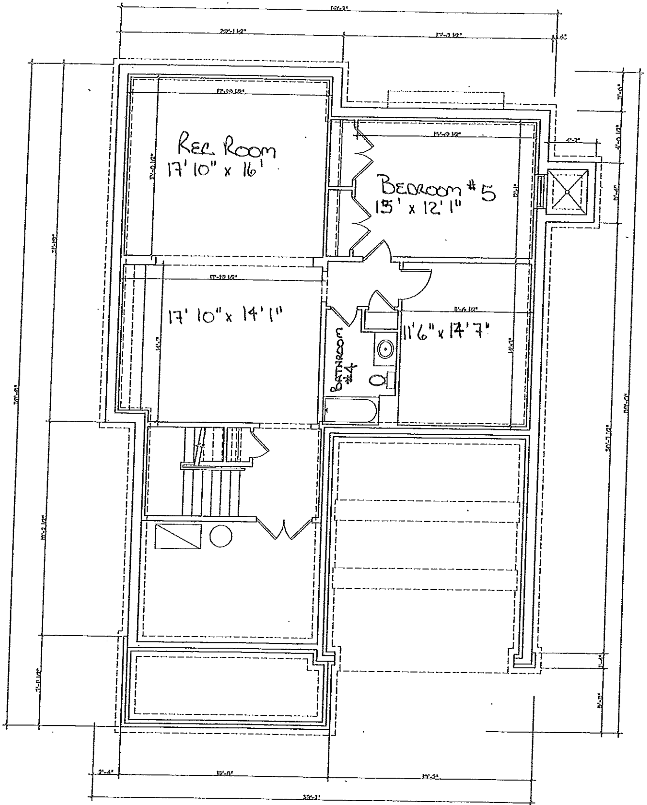
LOWER LEVEL PLAN
