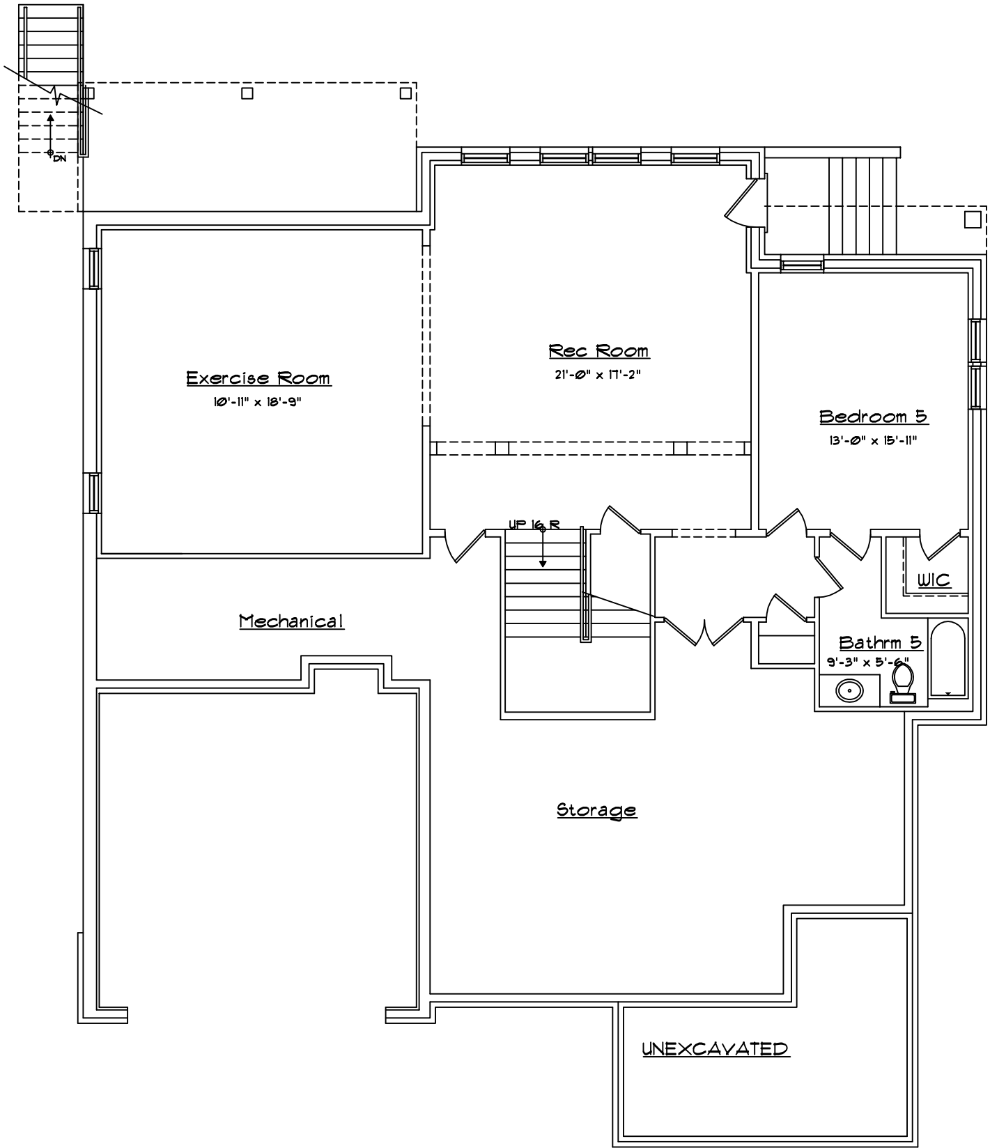
Lower Level Plan 1501 sf
