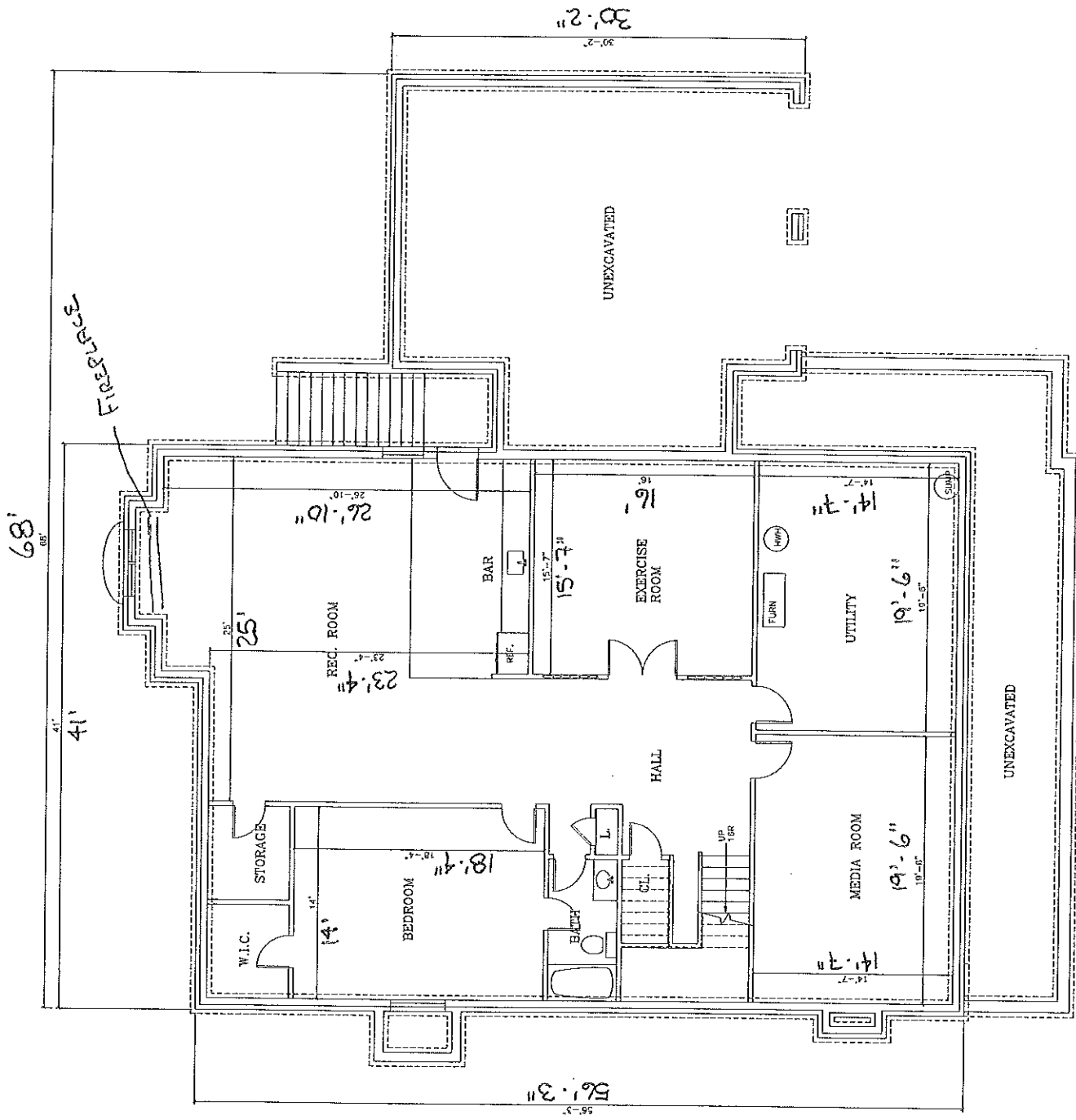
BASEMENT / FOUNDATION PLAN 1/4" = 1'-0"
