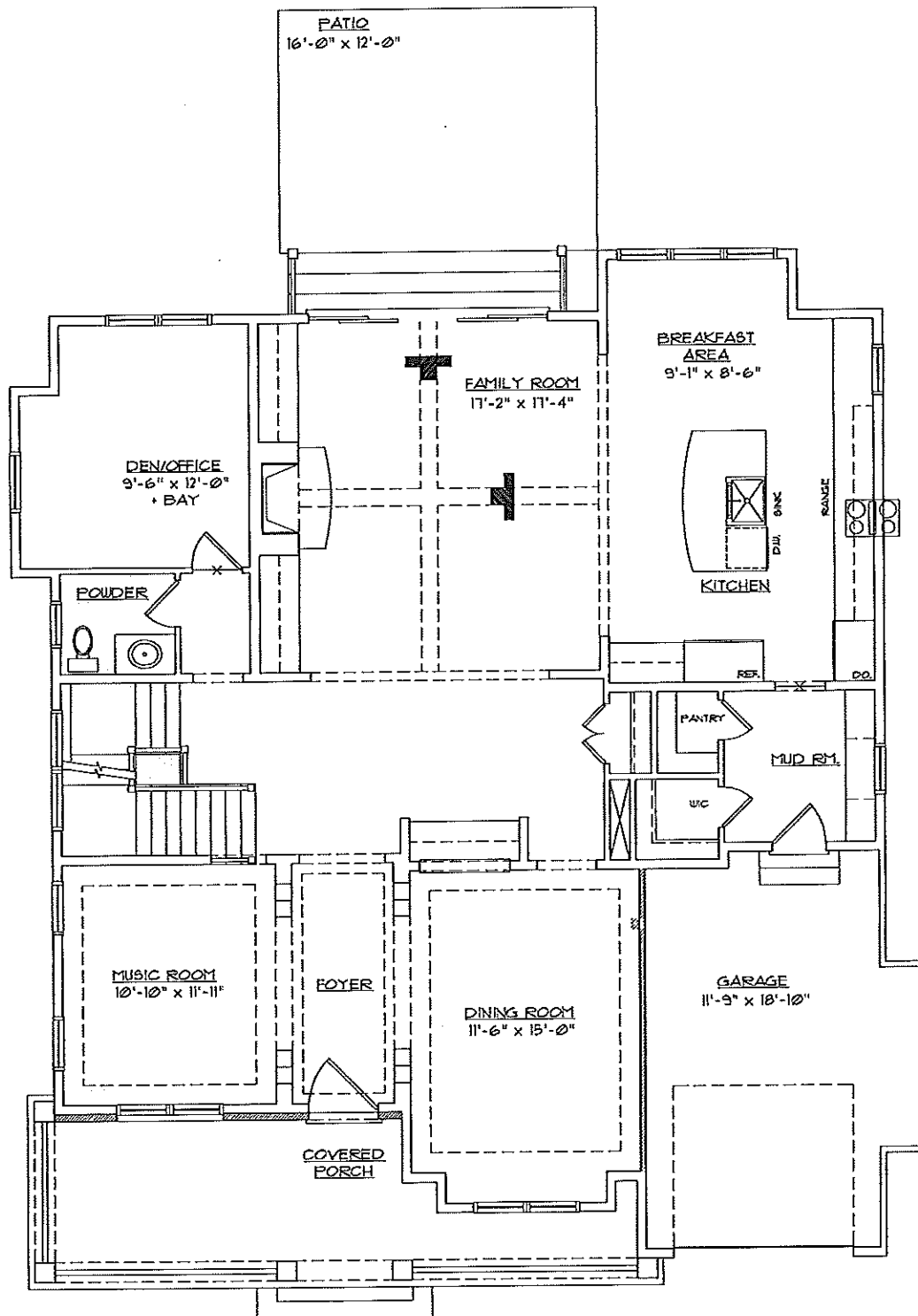
MAIN LEVEL
