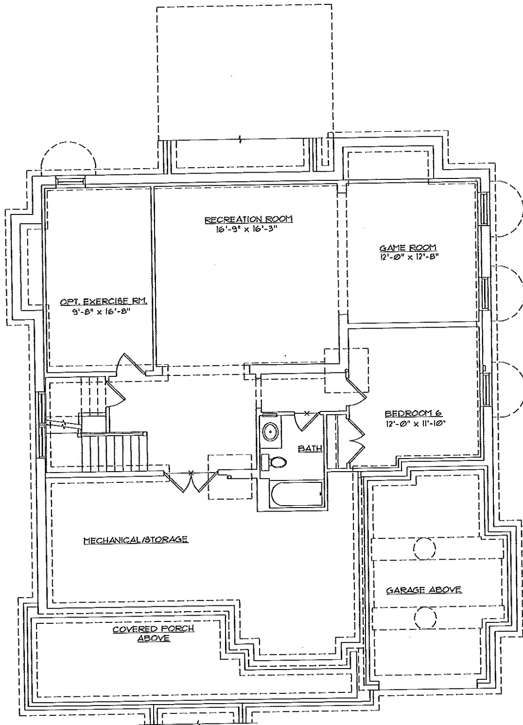
LOWER LEVEL
