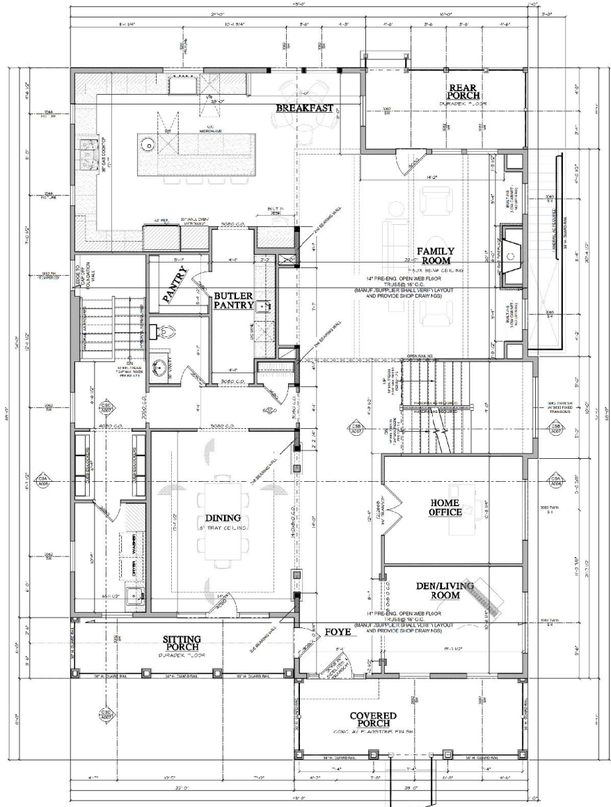
FIRST FLOOR PLAN SCALE: 1/4"=1'-0" 2,450 SQ. FT.
